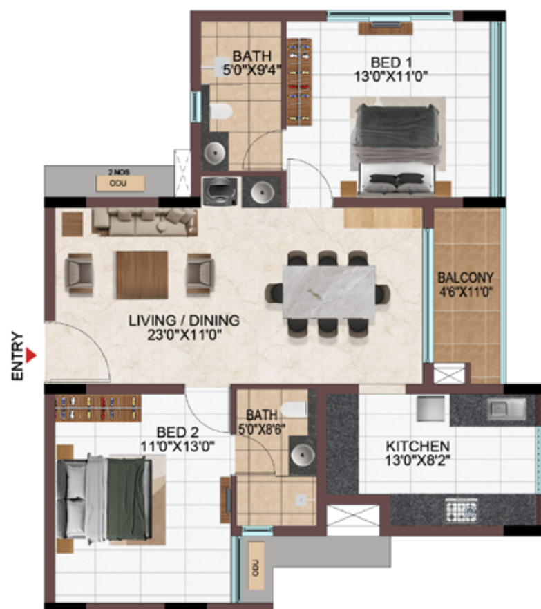
TYPICAL FLOOR ( 1 ST TO 9 TH )
