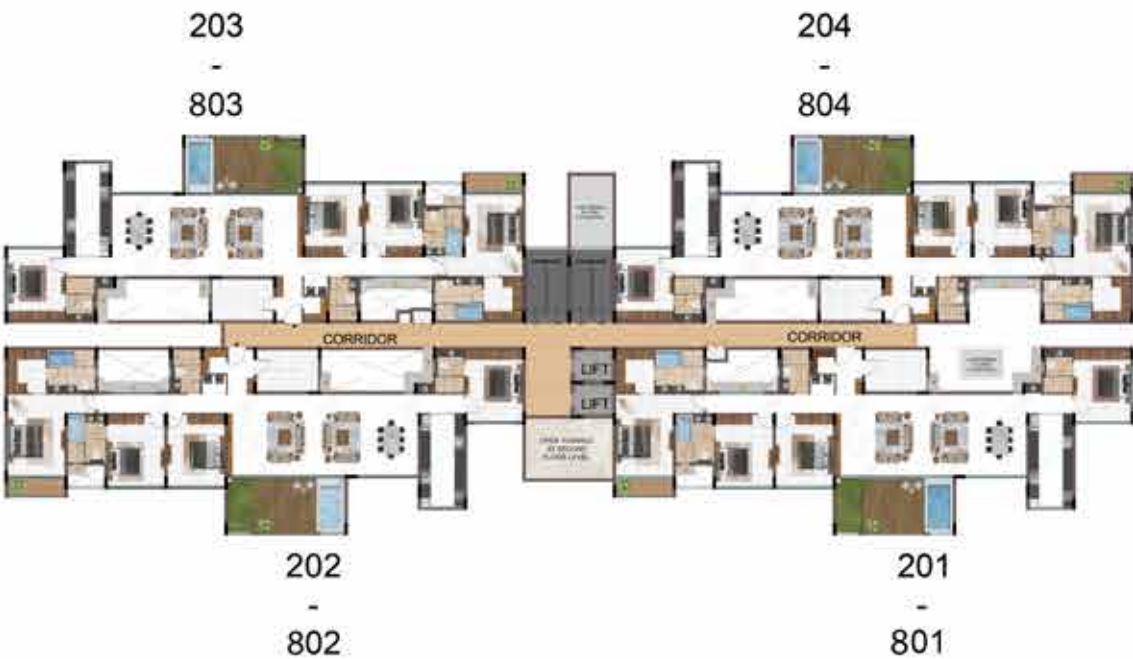
TYPICAL FLOOR (2 ND TO 8 TH )
